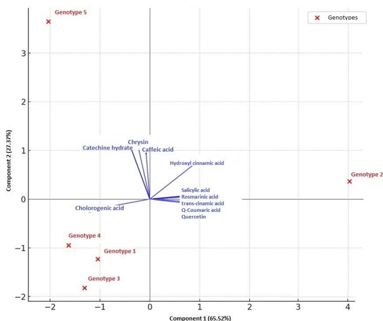
Figure 1. Principal component analysis (PCA) of phenolics.
